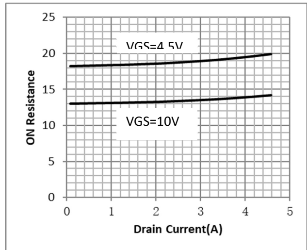
Fig.4 Resistance V gs vs Drain Current
